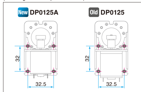
Mounting Hole Pitch Comparison (No changes from the previous model)
